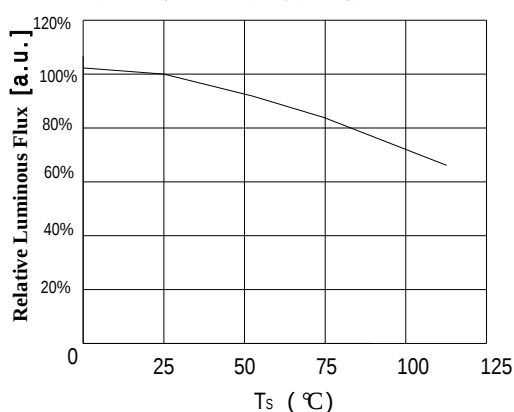
Case Temperature vs. Relative Luminous Flux 结点温度与相对流明曲线图 IF=3100mA
